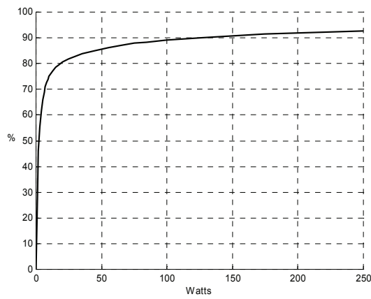
Figure 6: Efficiency vs. output power (8Ω).
