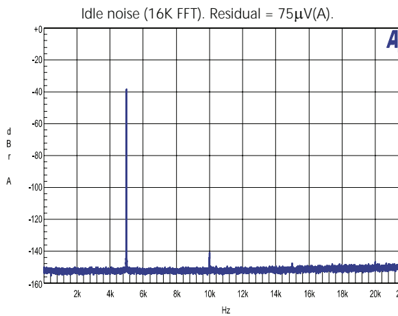
FFT Analysis. f = 5kHz/100mW 4Ω loading. THD = -101dB (0.0009%)
